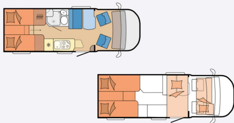
Grundriss: Hobby OPTIMA ONTOUR EDITION V65 GE 2024
